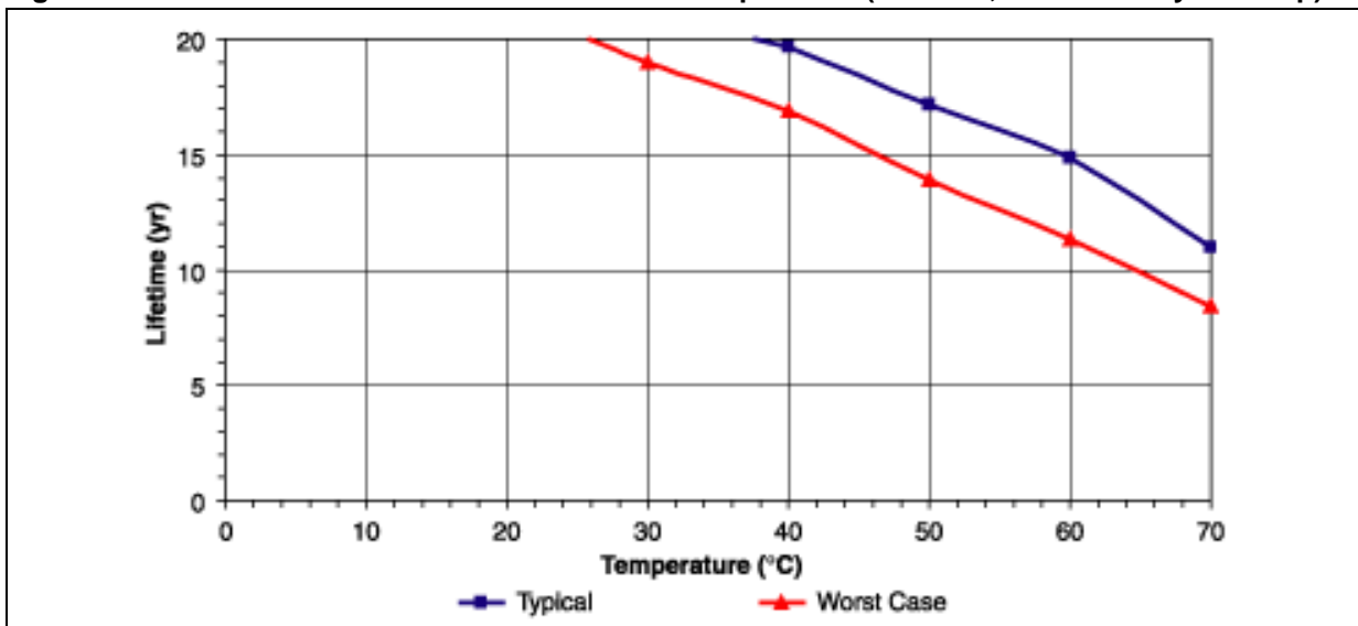
Figure 9. M48T58/59 Data Retention Lifetime vs. Temperature (120mAh, 100% Battery Back-up)
