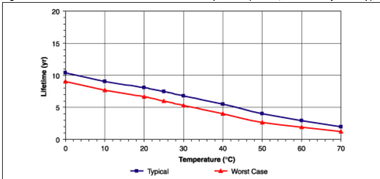
Figure 10. M48T35/37 Data Retention Lifetime vs. Temperature (48mAh, 100% Battery Back-up)
