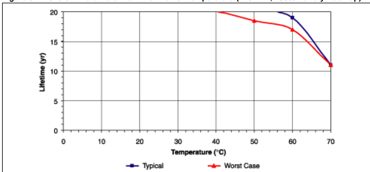
Figure 6. M48T02/12 Data Retention Lifetime vs. Temperature (120mAh, 100% Battery Back-up)
