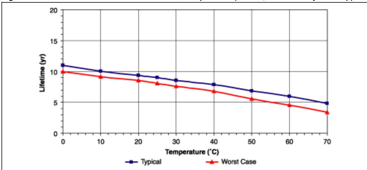
Figure 8. M48T58/59 Data Retention Lifetime vs. Temperature (48mAh, 100% Battery Back-up)
