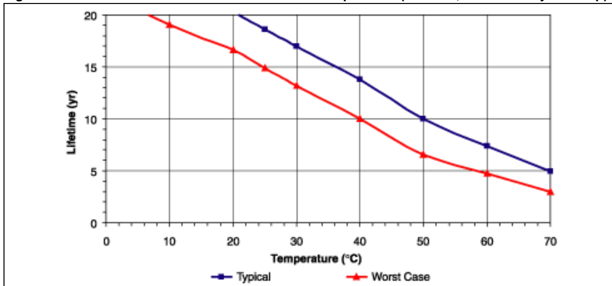
Figure 11. M48T35/37 Data Retention Lifetime vs. Temperature (120mAh, 100% Battery Back-up)
