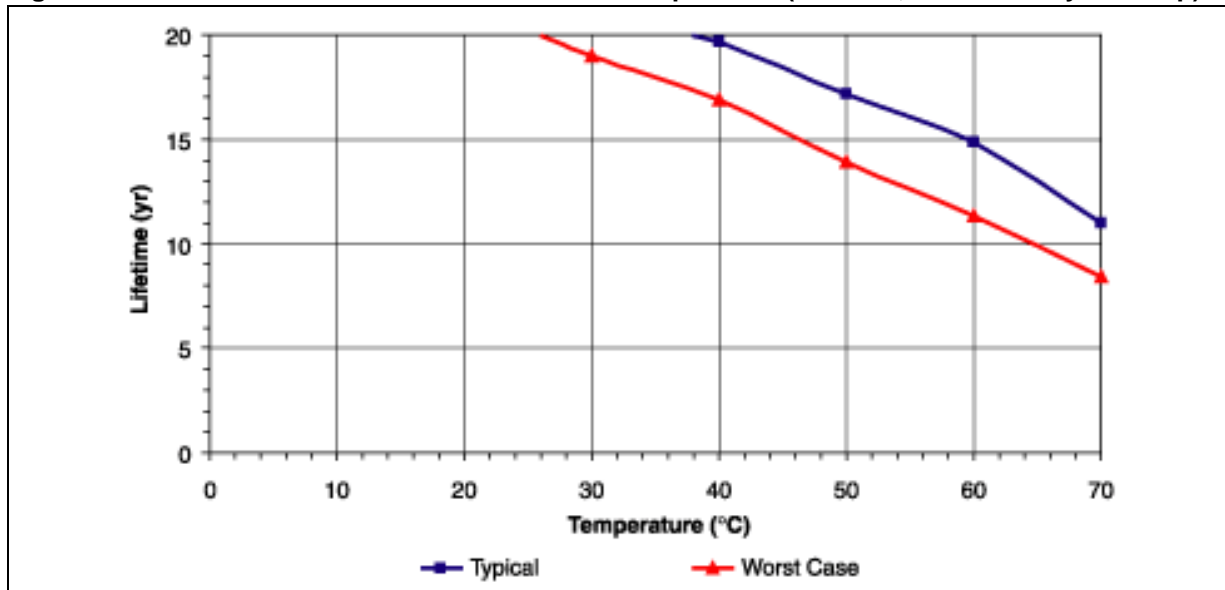
Figure 7. M48T08/18 Data Retention Lifetime vs. Temperature (120mAh, 100% Battery Back-up)
